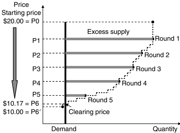
Figure 9.2. Aggregate supply curve
